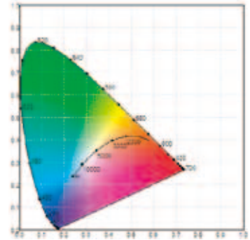
XY Chromaticity Diagram (CIE 1931 chromaticity diagram)
